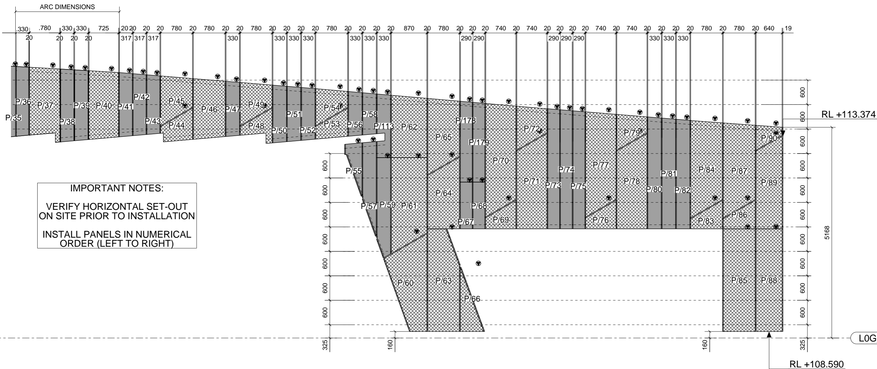
5b - ELEVATION B-B - LEISURE POOL
