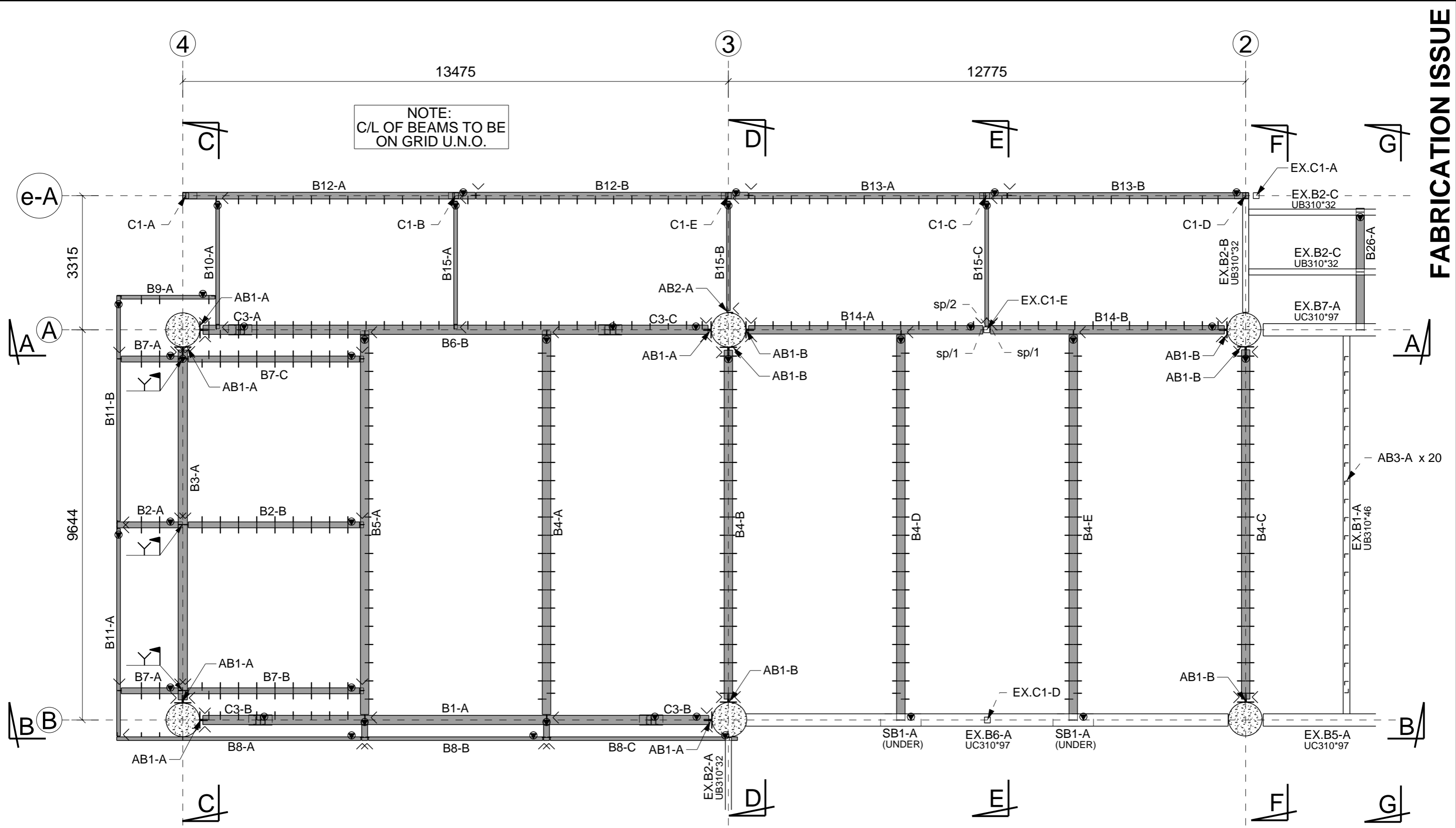
4a - MARKING PLAN - MEZZANINE FRAME
